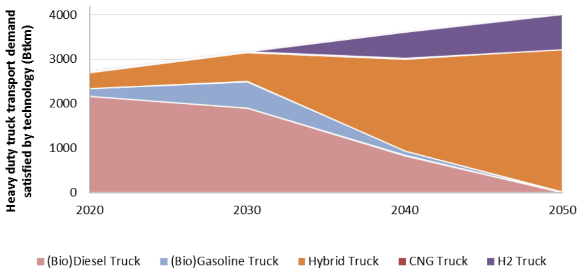
Figure 76 – Evolution of technology shares in freight trucks in HRES scenario
